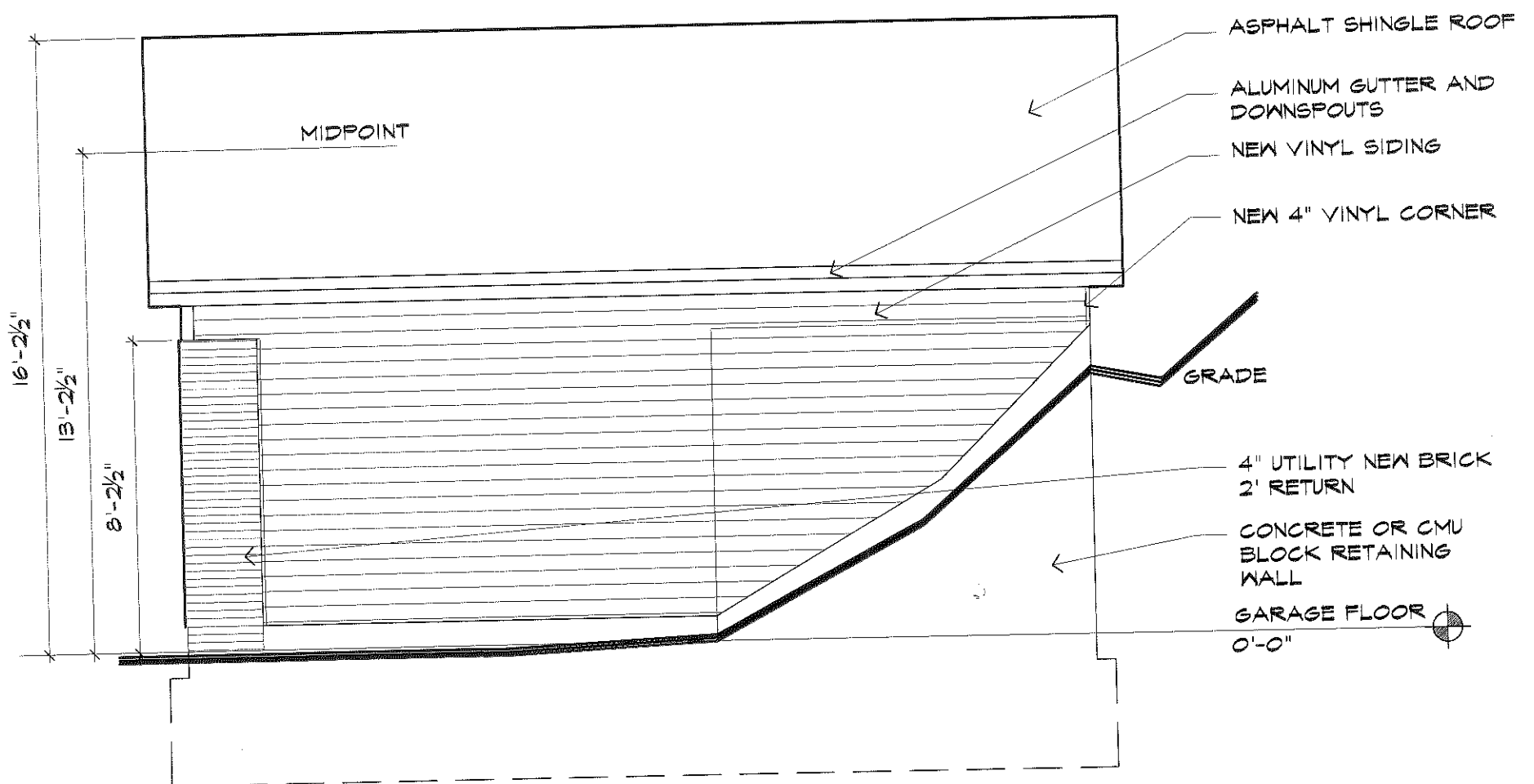
RIGHT (WEST) ELEVATION
