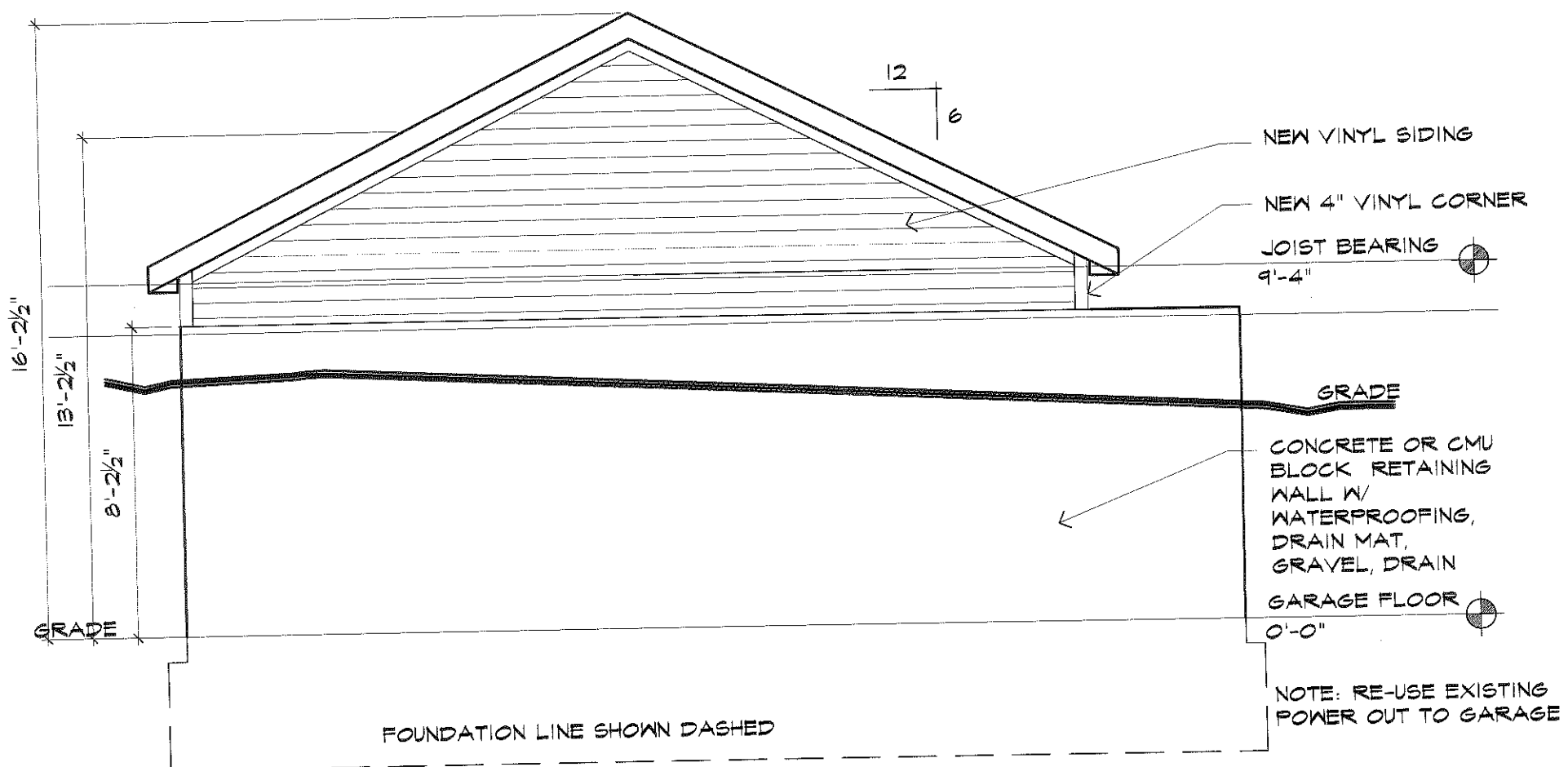
REAR (SOUTH) ELEVATION
