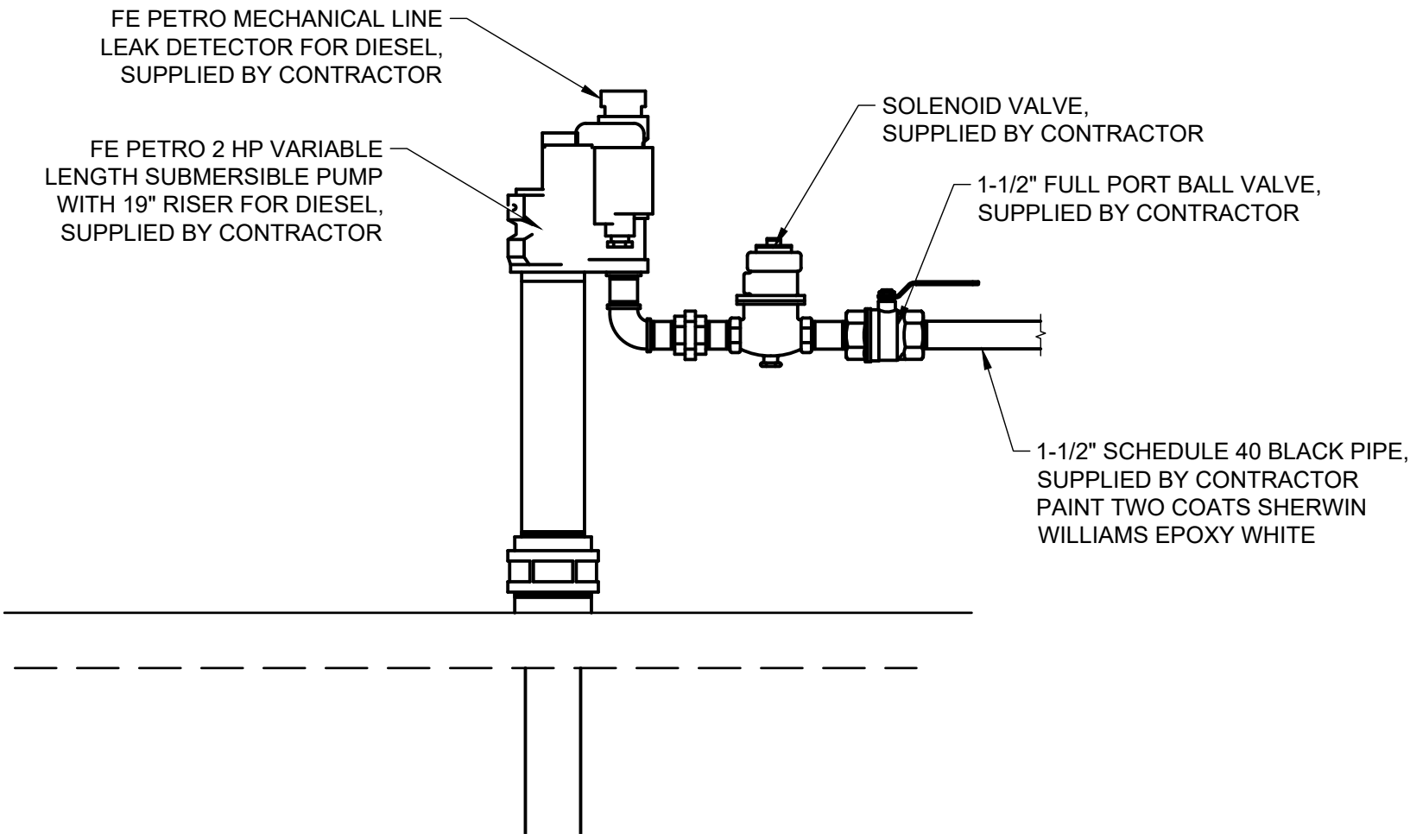
A DIESEL TANK STP INSTALLATION SCALE: 1" = 1'-0"
