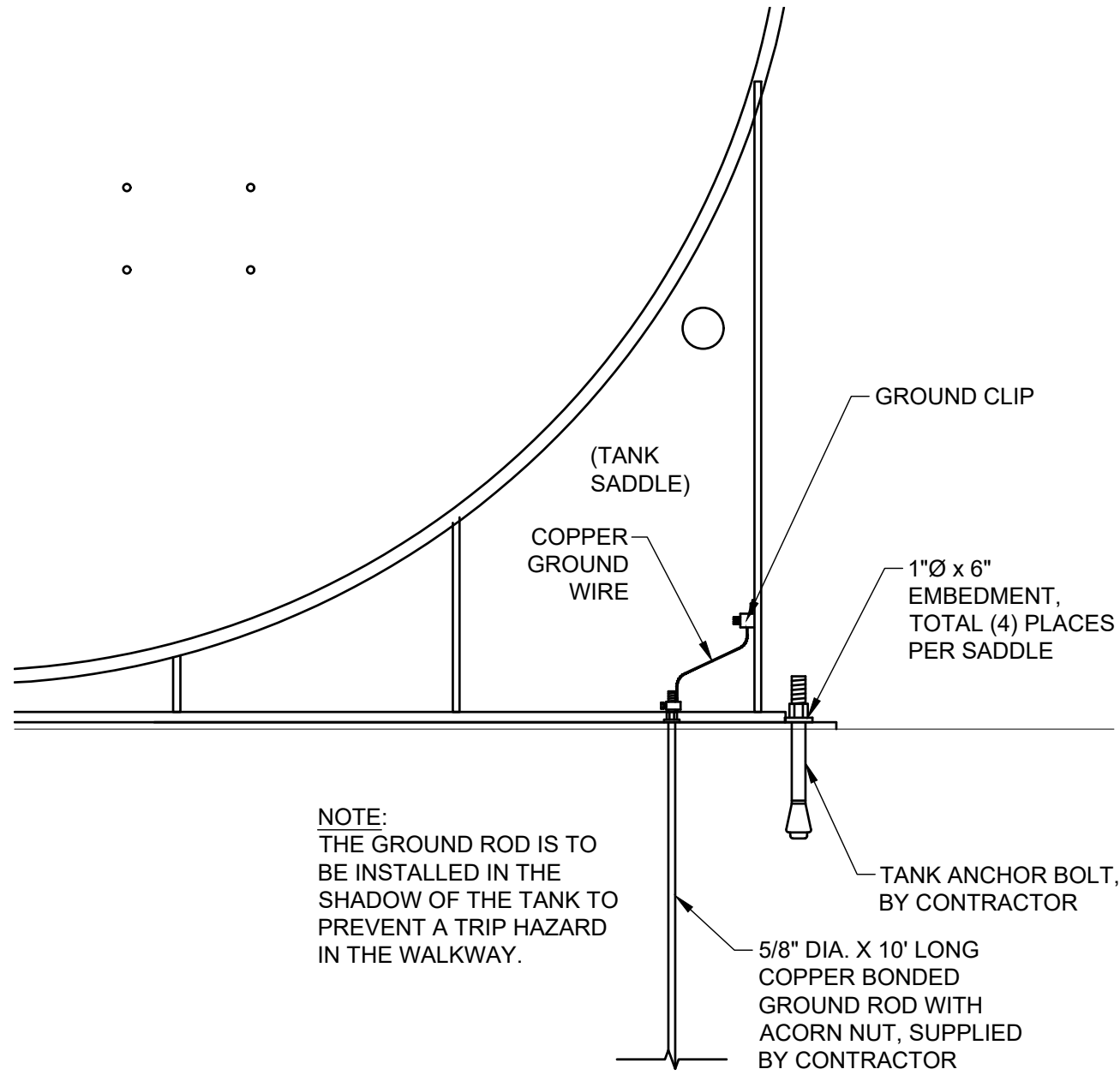
B TANK MOUNTING DETAIL SCALE: 1" = 1'-0"
