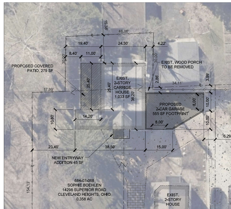
WORK AREA SITE PLAN SCALE: 1" = 20'
