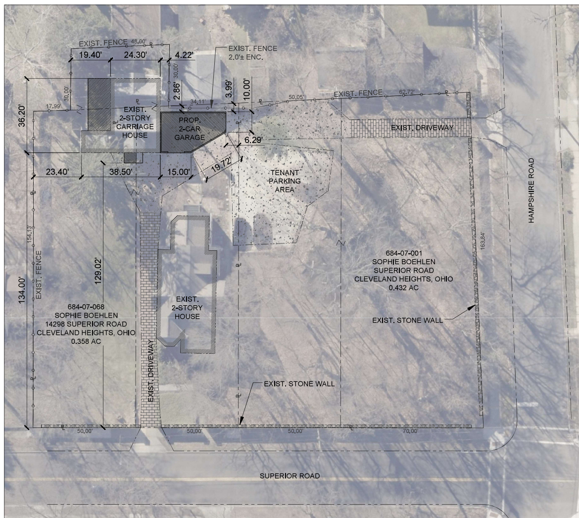
PROJECT SITE PLAN SCALE: 1" = 30'
